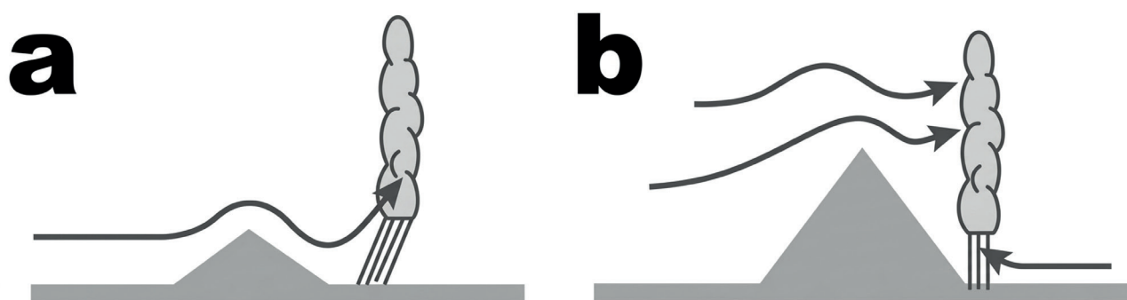
Fig. 8 As in Fig. 7, but showing: (a) downstream lee-wave convection initiated by ascent in the lee-wave crests downstream of hills or low mountains, and (b) upstream-tilted vertically propagating mountain waves over higher terrain. Figure adapted from Houze (1993, his Fig. 12.24; 2012, his Fig. 3) with permission.
