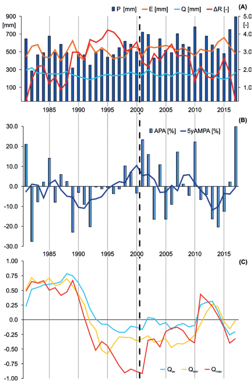
Fig. 4 The annual precipitation ( P ) at Płazowo site, annual sums of evaporation ( E ) (Okoniewska and Szumińska 2020), annual discharge ( Q ), and retention ( \Delta R ) presented using the method of integral curves for the years 1981–2017 (A), the precipitation anomaly (APA) for each year in the 1981–2017 period as a percentage relative to the long-term reference period of 1981–2010 (B), and the long-term trend of water discharge for the Tuchola gauging station for Q_{av} , Q_{max} and Q_{min} for the period 1981–2017 (C).
